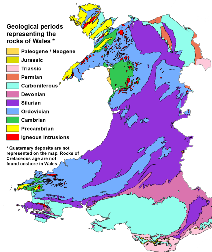
Figure 18 The geology map of Wales highlights the diverse nature of the underlying geology. Each colour represents rocks from the different geological periods. Contains British Geological Survey materials © NERC [2016].
