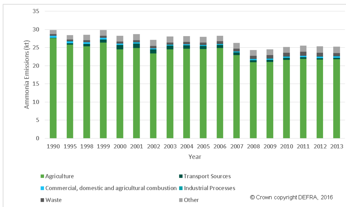
Figure 12 Wales Ammonia ( \text{NH}_3 ) Emissions by Source Sector 67
