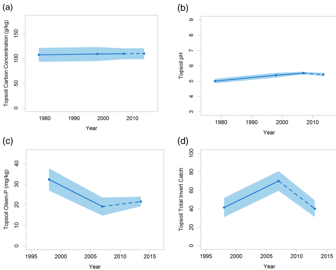
Figure 3.15 Glastir Monitoring and Evaluation Programme (GMEP) data for topsoil: (a) Long term trends in carbon concentration (1978 to 2013); (b) Long term trends in topsoil pH; (c) Long term trends in topsoil phosphorus availability (Olsen-P); (d) Trend in topsoil mesofauna abundance. Solid blue line = Countryside Survey data (CS data); Dashed blue line = GMEP 2013 Wider Wales Survey 72 . [M]
