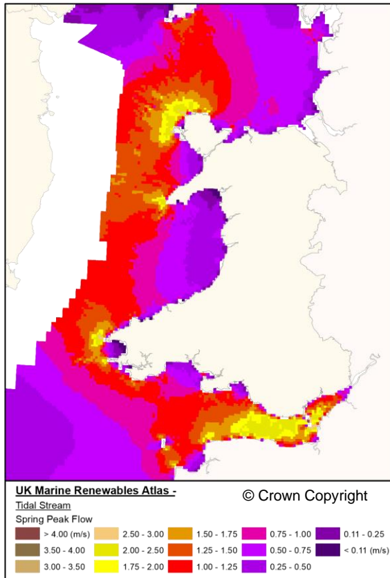
Figure 3.10 Map of peak spring tidal flow for Welsh waters reproduced from: Atlas of UK Marine Renewable Energy Resources (2008) 57 . [H]
