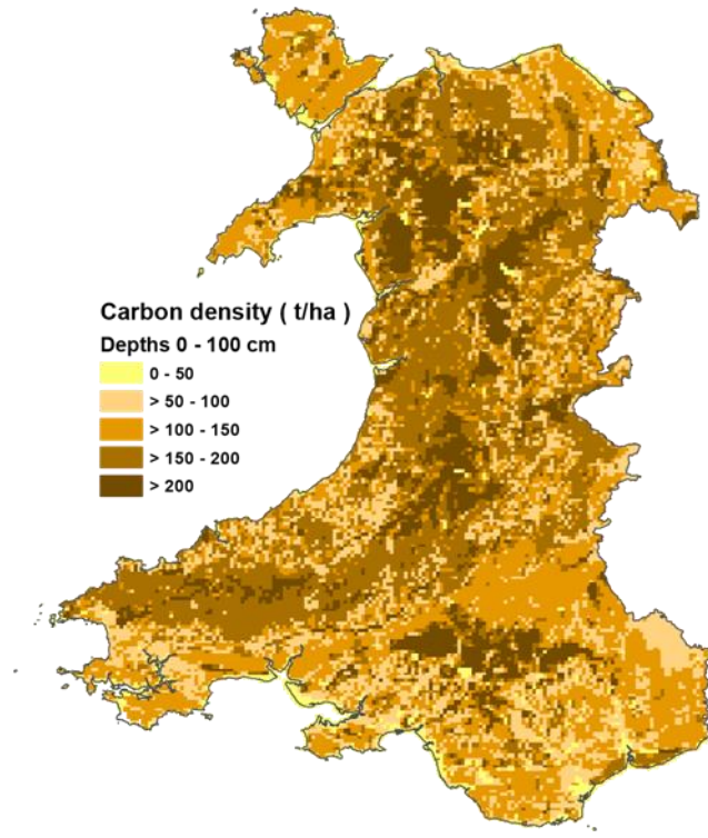
Figure 3.13 Distribution of soil carbon in Wales, shown as carbon density (t/ha): a) depth 0-30 cm; b) depth 30-100 cm; c) depth 0-100 cm 79 .
