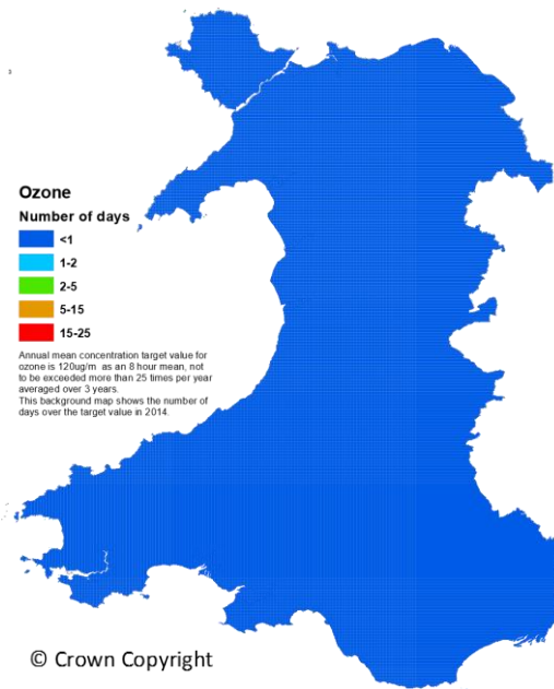
Figure 3.7 Number of days background ozone concentration was over target value in 2014 41 . [M]
