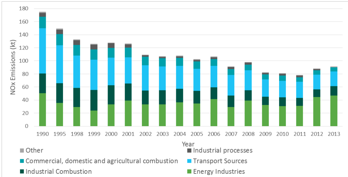
Figure 3.6 Wales nitrogen oxides (NOx) emissions by source sector 37 . [H]
