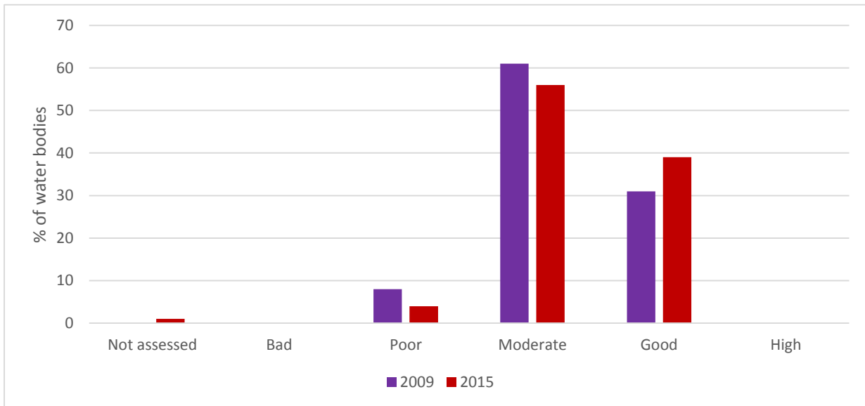
Figure 11. Percentage comparison between ecological classification for surface water between 2009 and 2015.
