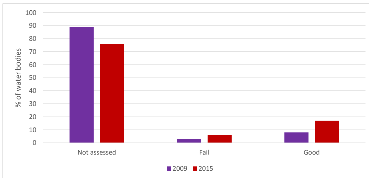
Figure 9. Comparison of 2009 and 2015 chemical classification
