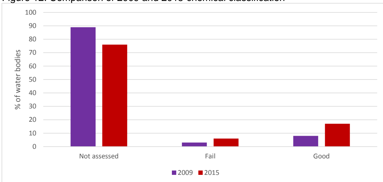
Figure 12. Comparison of 2009 and 2015 chemical classification
