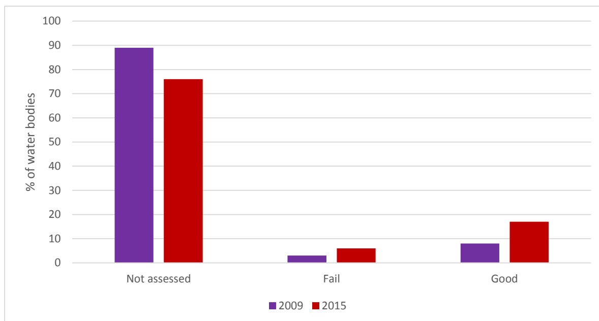
Figure 6. Graph showing comparison between chemical classification for surface water between 2009 and 2015.
