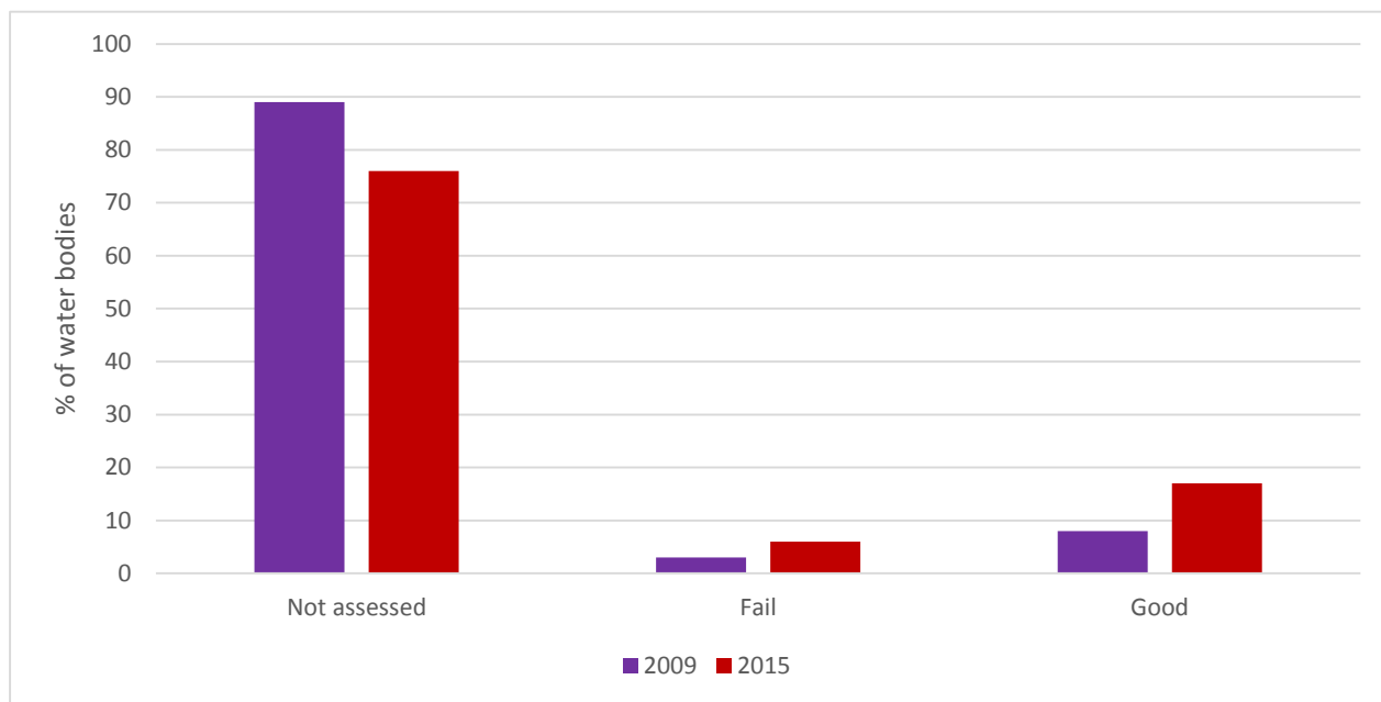
Figure 3. Percentage comparison between chemical classification for surface water between 2009 and 2015.
