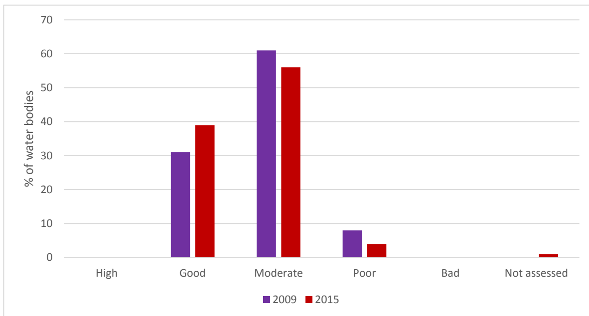
Figure 5. Graph showing percentage comparison between ecological classification for surface water between 2009 and 2015.
