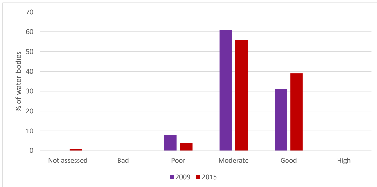
Figure 8. Percentage comparison between ecological classification for surface water between 2009 and 2015.
