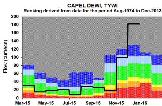
Figure 14: River Flow Charts: South West Wales
