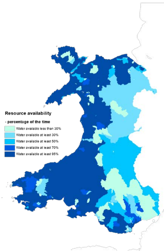
Figure 3.9 Water resource availability in Wales in 2014 (percentage of time) 45, 46 . [H]
